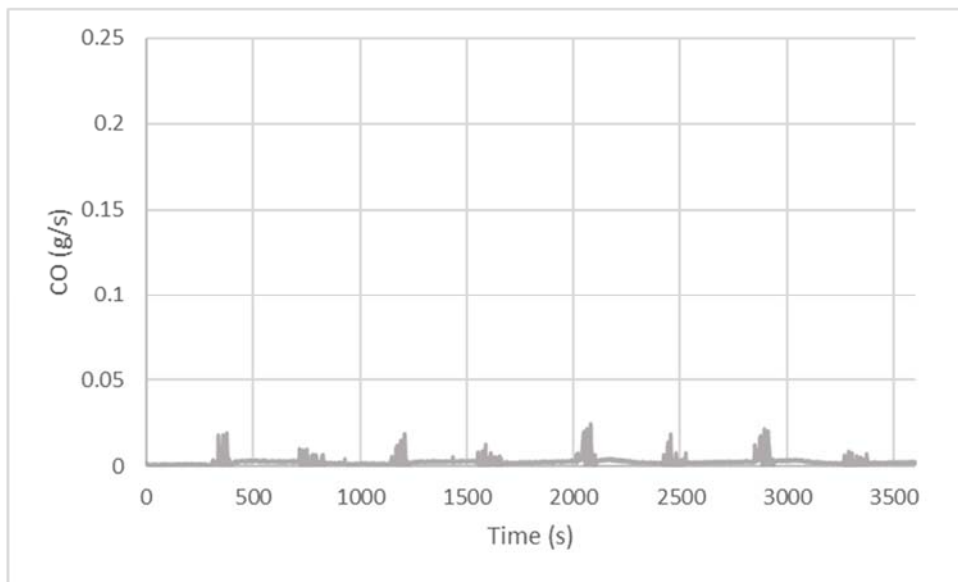
Figure 81: Mass Rate (g/s) of CO Emissions for 2017 Diesel School Bus from 5 Minute Stop and Go Route
