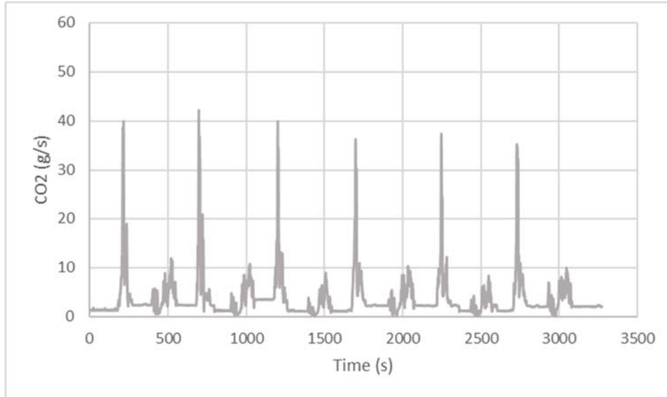
Figure 48: Mass Rate (g/s) of CO 2 Emissions for Diesel School Bus from Stop and Go Route
