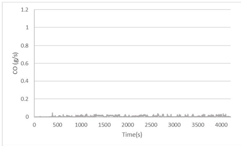
Figure 58: Mass Rate (g/s) of CO Emissions for 2017 Diesel School Bus from Cold Morgantown Route
