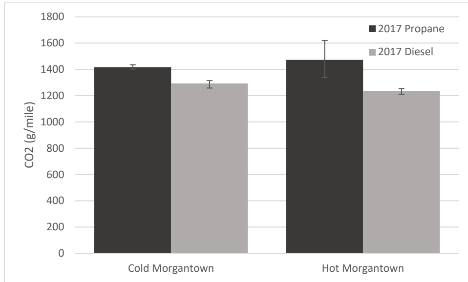
Figure 61: Average CO 2 Emissions (g/mile) for 2017 Propane and 2017 Diesel School Bus
