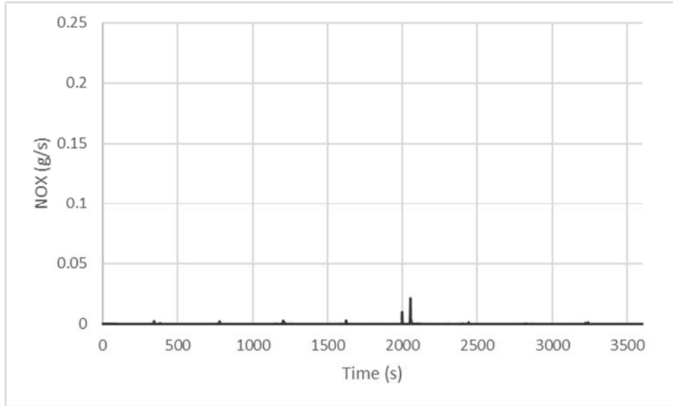
Figure 95: Mass Rate (g/s) of NOX Emissions for 2017 Propane School Bus from 5 Minute Stop and Go Route
