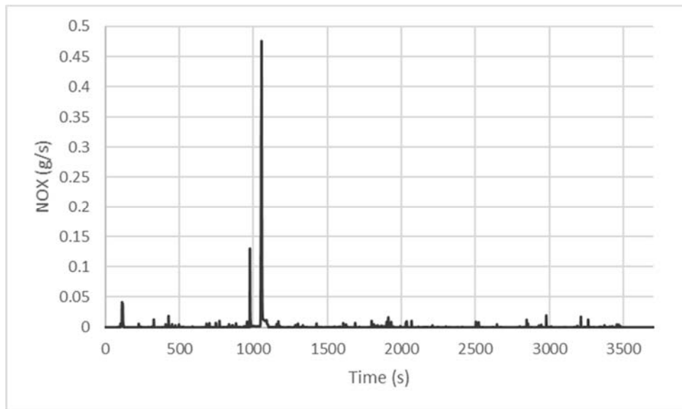
Figure 74: Mass Rate (g/s) of NO x Emissions for 2017 Propane School Bus from Hot Morgantown Route
