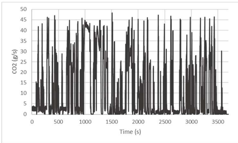
Figure 64: Mass Rate (g/s) of CO 2 Emissions for 2017 Propane School Bus from Hot Morgantown Route
