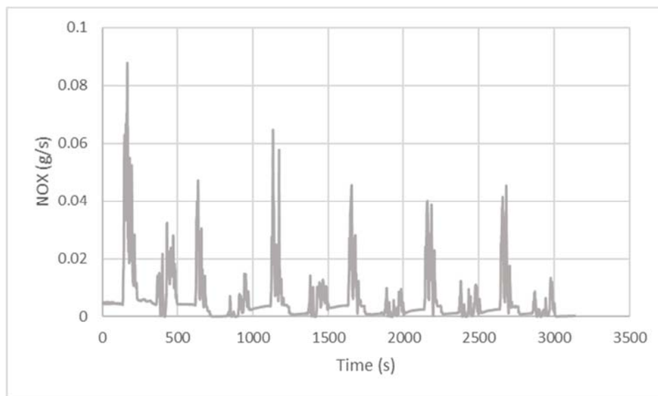
Figure 54: Mass Rate (g/s) of NO x Emissions for Diesel School Bus from Stop and Go Route
