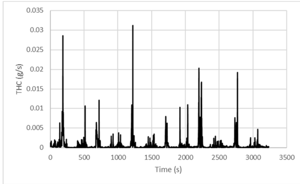
Figure 50: Mass Rate (g/s) of THC Emissions for Propane School Bus from Stop and Go Route
