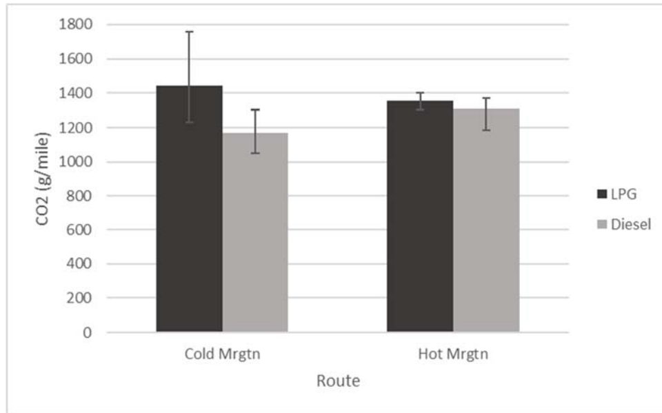
Figure 27: Average CO 2 Emissions (g/mile) for Propane and Diesel School Bus
