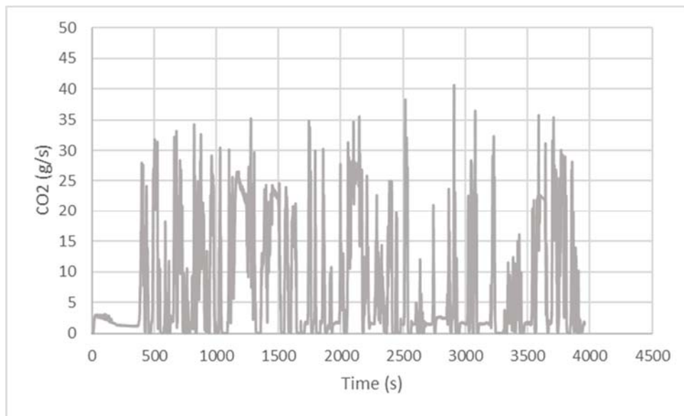
Figure 29: Mass Rate (g/s) of CO 2 Emissions for Diesel School Bus from Cold Morgantown Route
