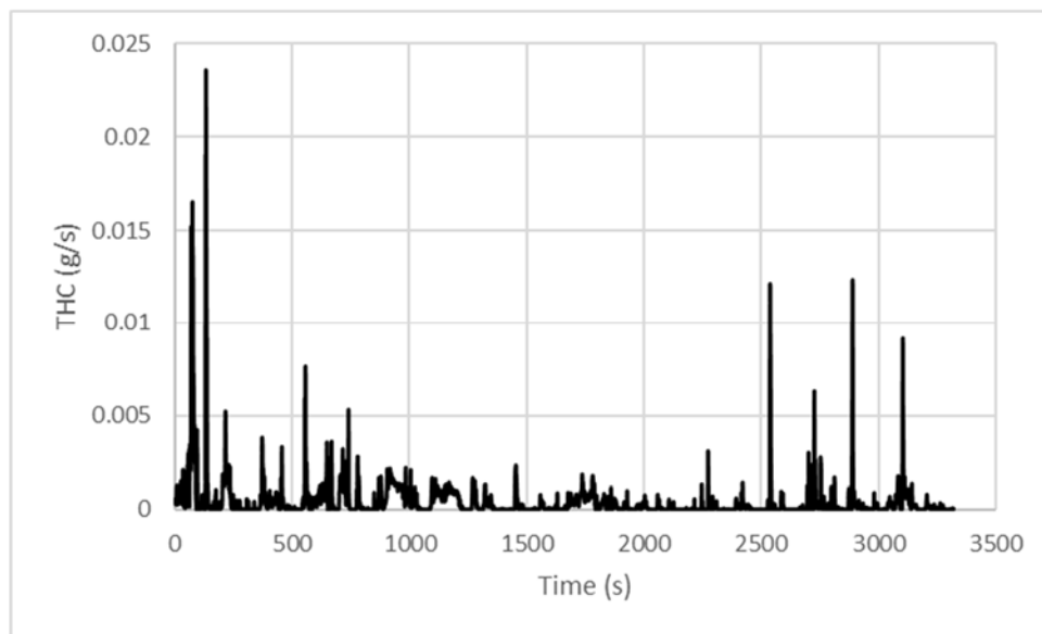
Figure 35: Mass Rate (g/s) of THC Emissions for Propane School Bus from Hot Morgantown Route
