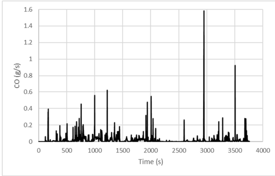
Figure 25: Mass Rate (g/s) of CO Emissions for Propane School Bus from Hot Morgantown Route
