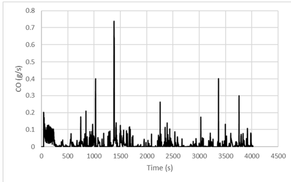
Figure 23: Mass Rate (g/s) of CO Emissions for Propane School Bus from Cold Morgantown Route
