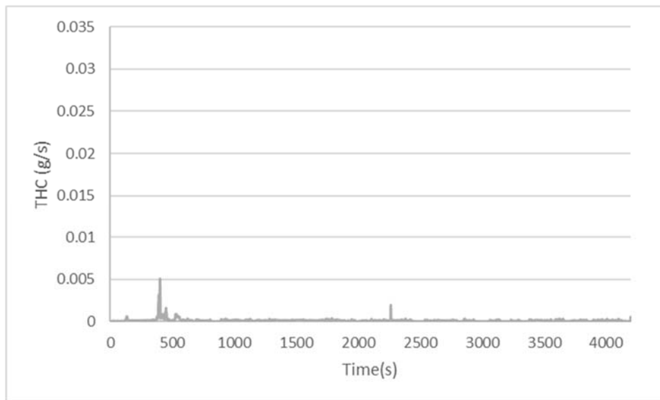
Figure 68: Mass Rate (g/s) of THC Emissions for 2017 Diesel School Bus from Cold Morgantown Route
