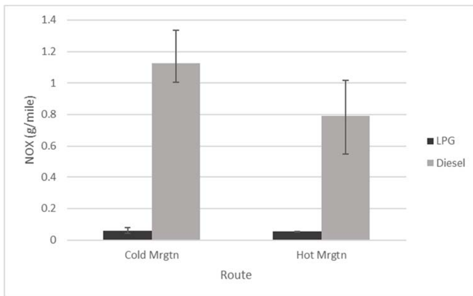
Figure 37: Average NO x Emissions (g/mile) for Propane and Diesel School Bus
