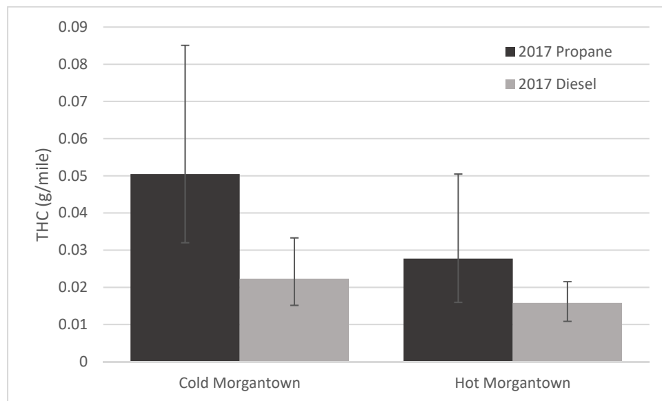
Figure 66: Average THC Emissions (g/mile) for 2017 Propane and 2017 Diesel School Bus
