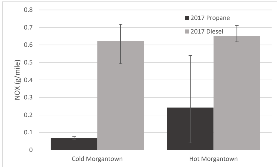
Figure 71: Average NO x Emissions (g/mile) for 2017 Propane and 2017 Diesel School Bus
