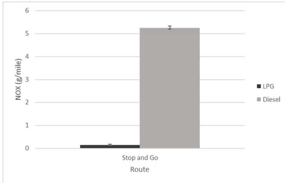
Figure 52: Average NO x Emissions (g/mile) for Propane and Diesel School Bus
