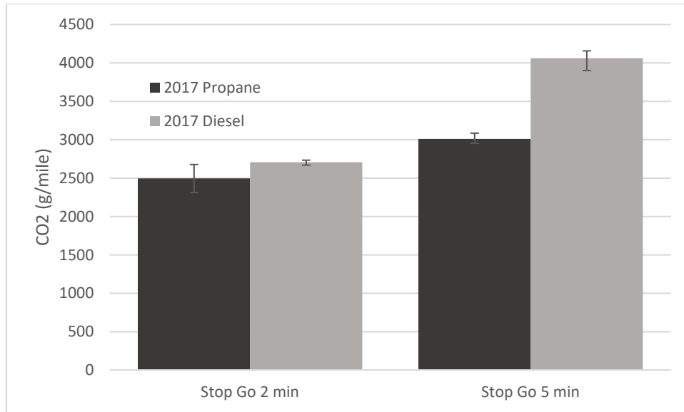
Figure 82: Average CO 2 Emissions (g/mile) for 2017 Propane and 2017 Diesel School Bus
