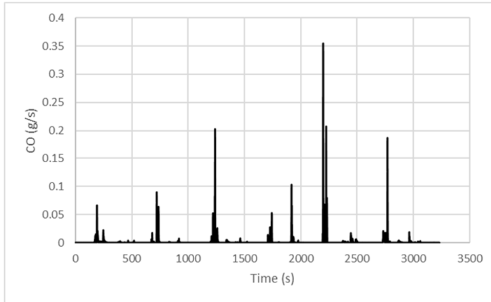
Figure 44: Mass Rate (g/s) of CO Emissions for Propane School Bus from Stop and Go Route
