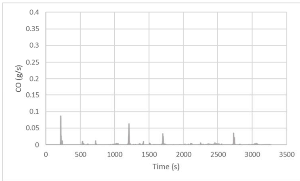
Figure 45: Mass Rate (g/s) of CO Emissions for Diesel School Bus from Stop and Go Route
