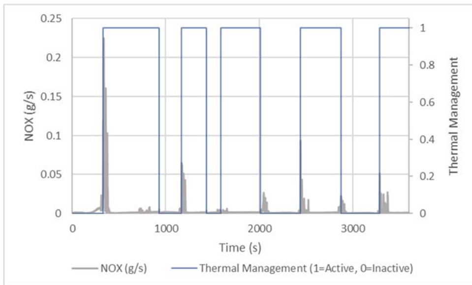
Figure 96: Mass Rate (g/s) of NOX Emissions for 2017 Diesel School Bus from 5 Minute Stop and Go Route
