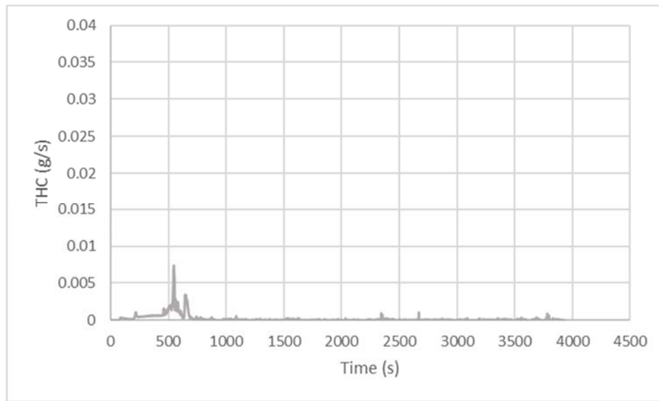
Figure 34: Mass Rate (g/s) of THC Emissions for Diesel School Bus from Cold Morgantown Route
