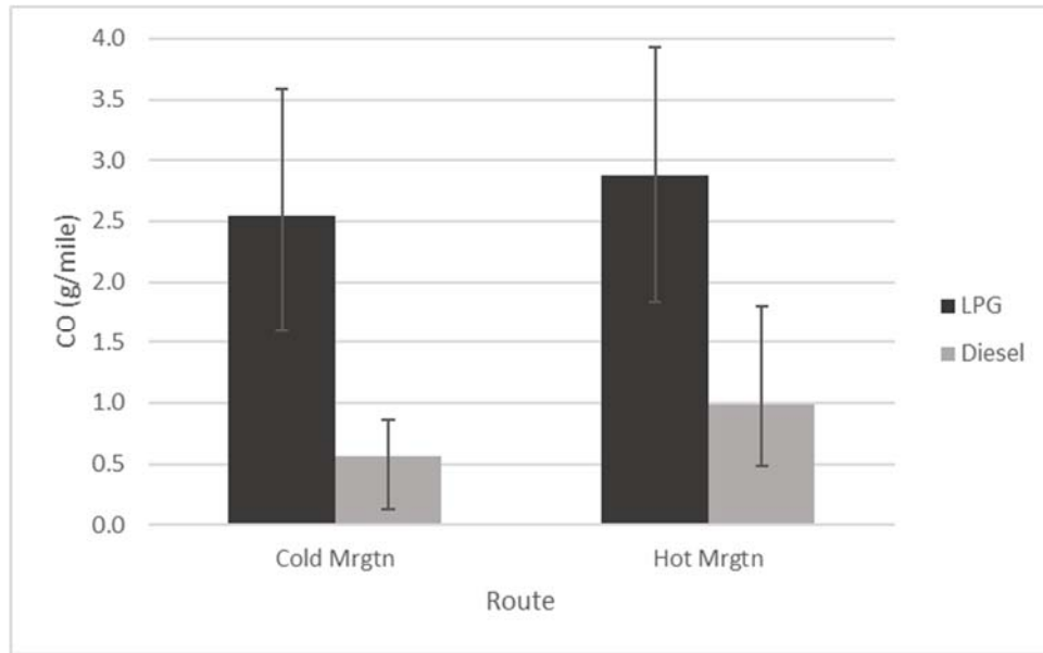
Figure 22: Average CO Emissions (g/mile) for Propane and Diesel School Bus
