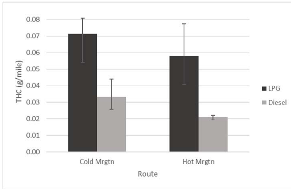
Figure 32: Average THC Emissions (g/mile) for Propane and Diesel School Bus
