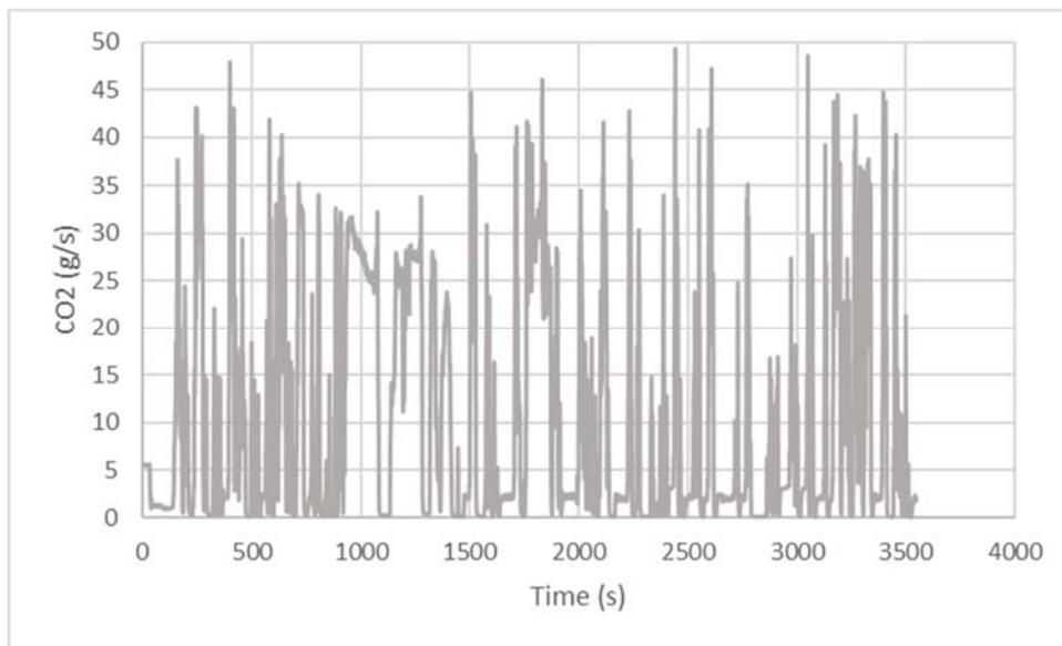
Figure 31: Mass Rate (g/s) of CO 2 Emissions for Diesel School Bus from Hot Morgantown Route
