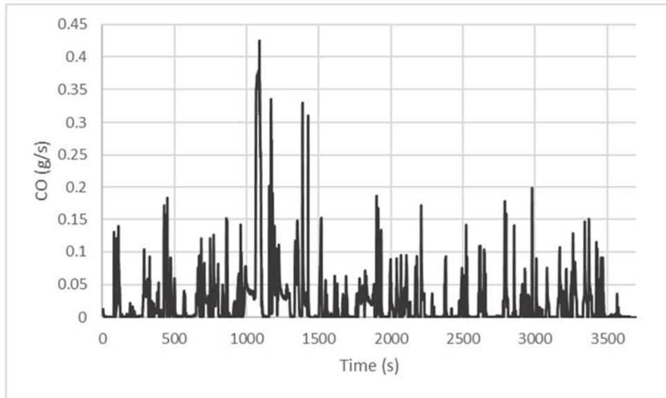
Figure 59: Mass Rate (g/s) of CO Emissions for 2017 Propane School Bus from Hot Morgantown Route
