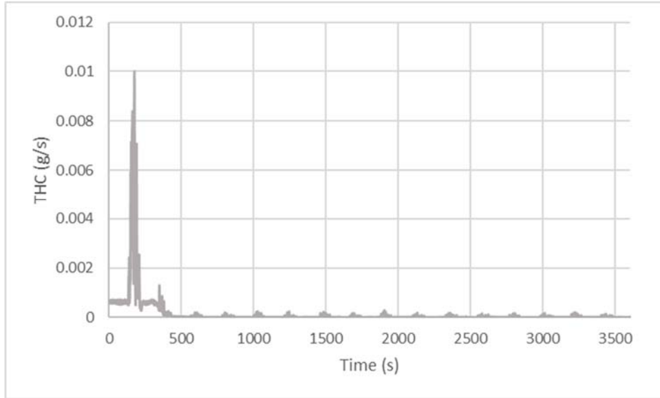
Figure 89: Mass Rate (g/s) of THC Emissions for 2017 Diesel School Bus from 2 Minute Stop and Go Route
