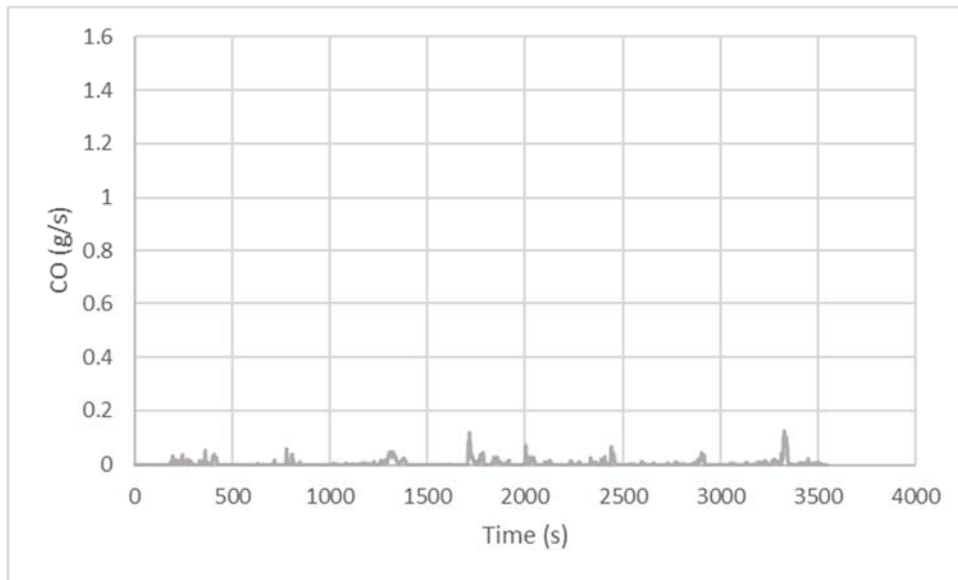
Figure 26: Mass Rate (g/s) of CO Emissions for Diesel School Bus from Hot Morgantown Route
