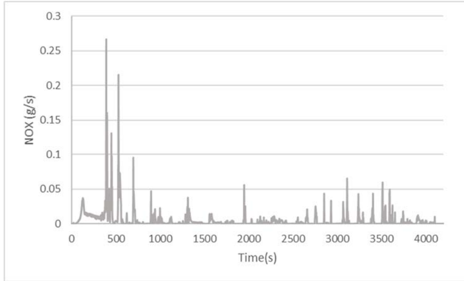
Figure 73: Mass Rate (g/s) of NO x Emissions for 2017 Diesel School Bus from Cold Morgantown Route
