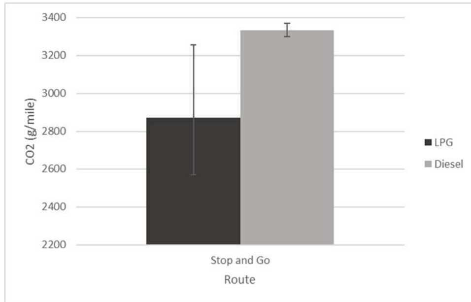
Figure 46: Average CO 2 Emissions (g/mile) for Propane and Diesel School Bus
