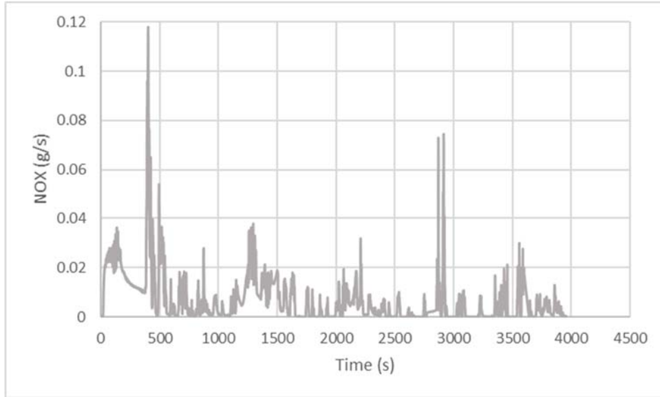
Figure 39: Mass Rate (g/s) of NO x Emissions for Diesel School Bus from Cold Morgantown Route
