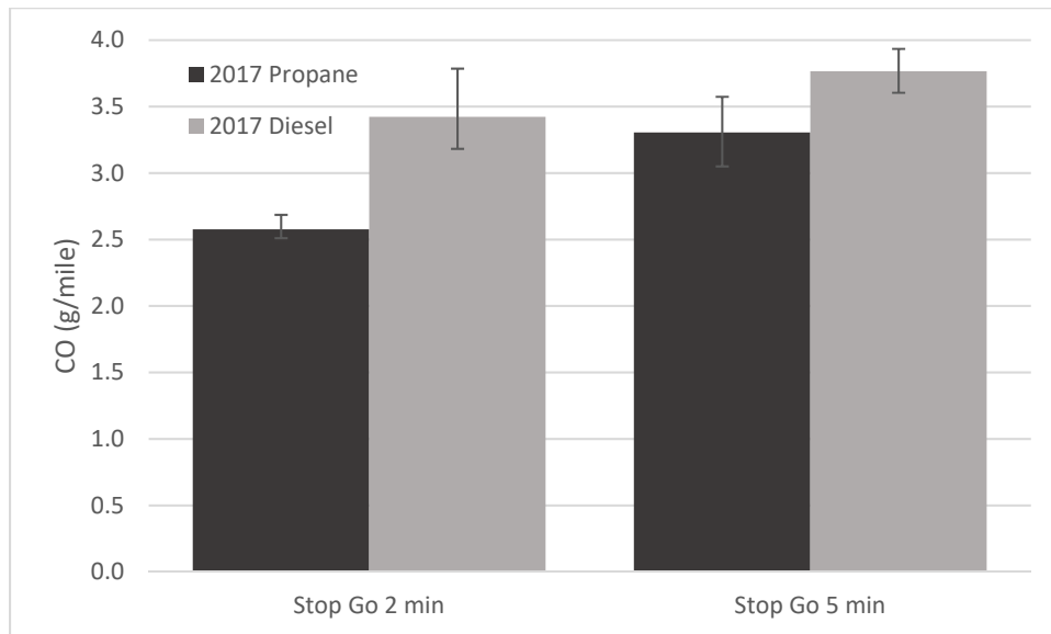
Figure 77: Average CO Emissions (g/mile) for 2017 Propane and 2017 Diesel School Bus
