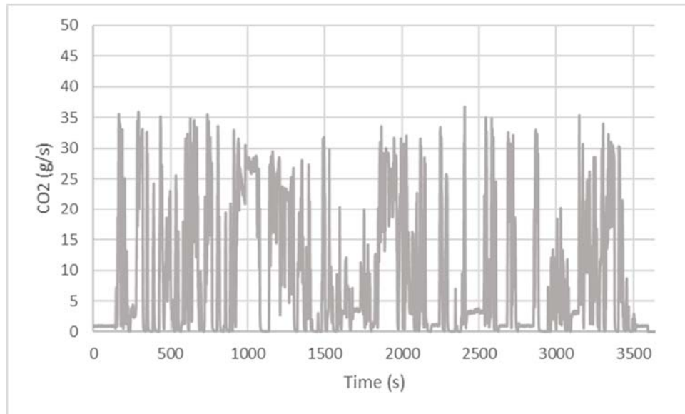
Figure 65: Mass Rate (g/s) of CO 2 Emissions for 2017 Diesel School Bus from Hot Morgantown Route
