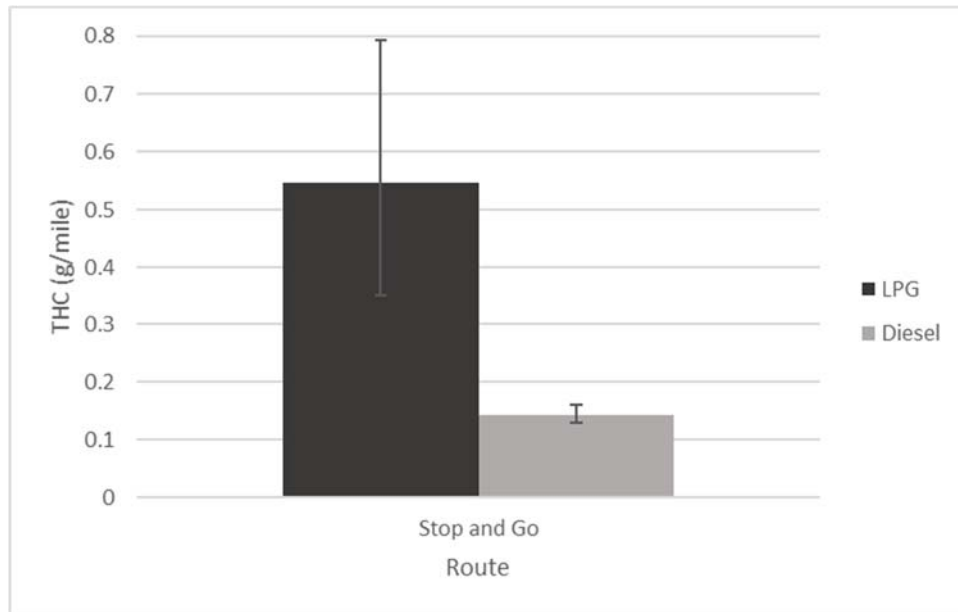
Figure 49: Average THC Emissions (g/mile) for Propane and Diesel School Bus
