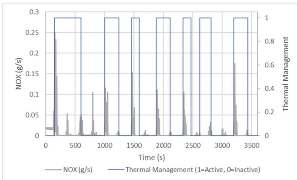
Figure 94: Mass Rate (g/s) of NO x Emissions for 2017 Diesel School Bus from 2 Minute Stop and Go Route
