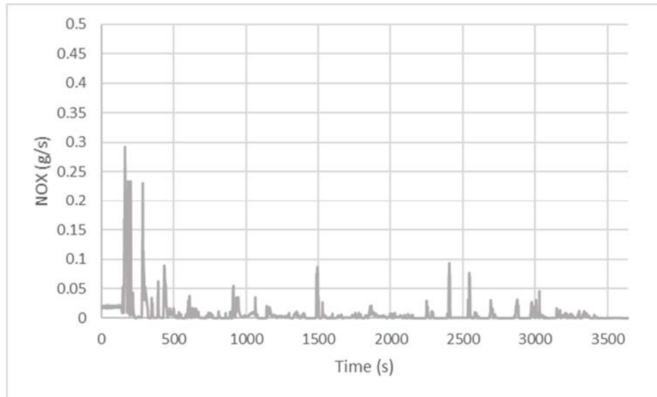
Figure 75: Mass Rate (g/s) of NO x Emissions for 2017 Diesel School Bus from Hot Morgantown Route
