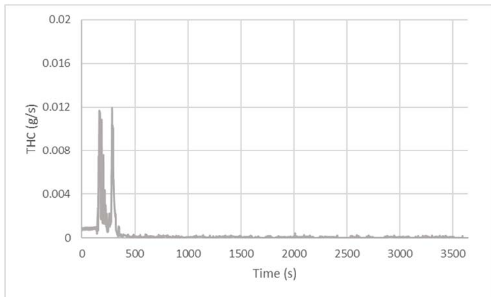
Figure 70: Mass Rate (g/s) of THC Emissions for 2017 Diesel School Bus from Hot Morgantown Route
