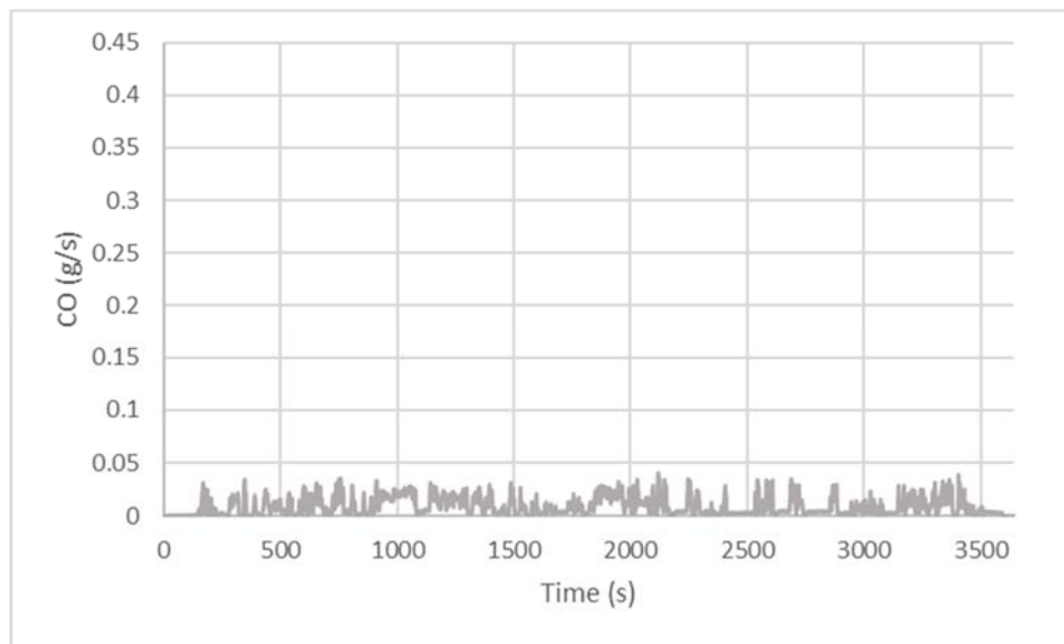
Figure 60: Mass Rate (g/s) of CO Emissions for 2017 Diesel School Bus from Hot Morgantown Route
