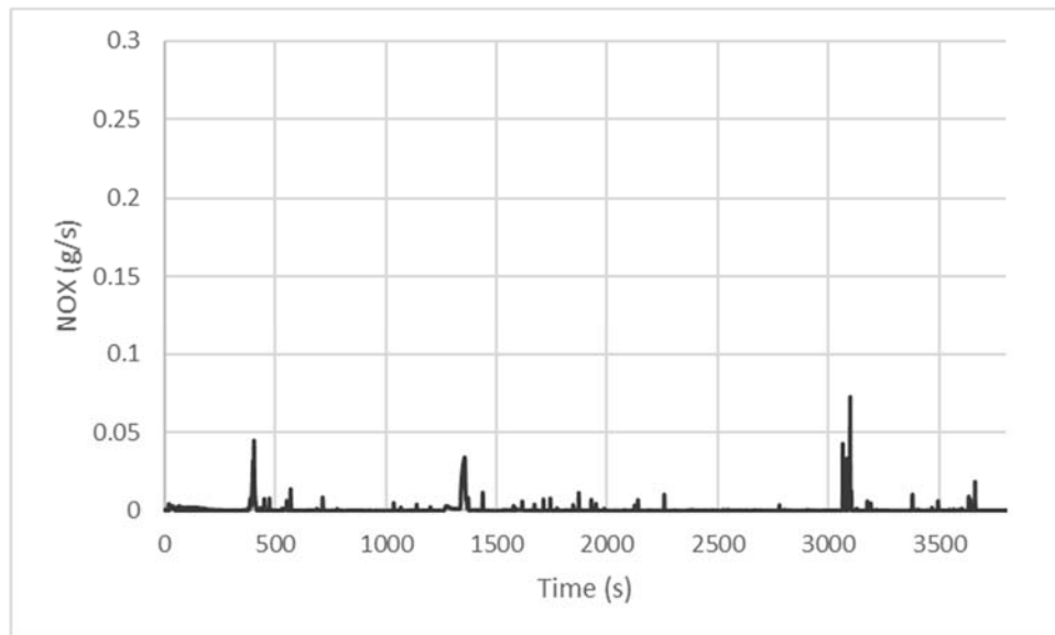
Figure 72: Mass Rate (g/s) of NO x Emissions for 2017 Propane School Bus from Cold Morgantown Route
