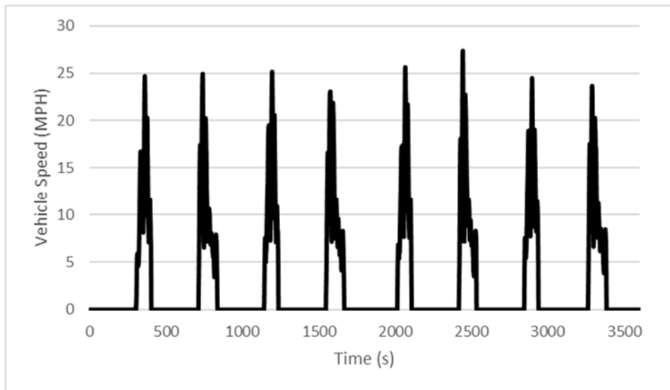
Figure 18: Characteristic Vehicle Speed Trace for the Stop and Go Route (5 Minute)
