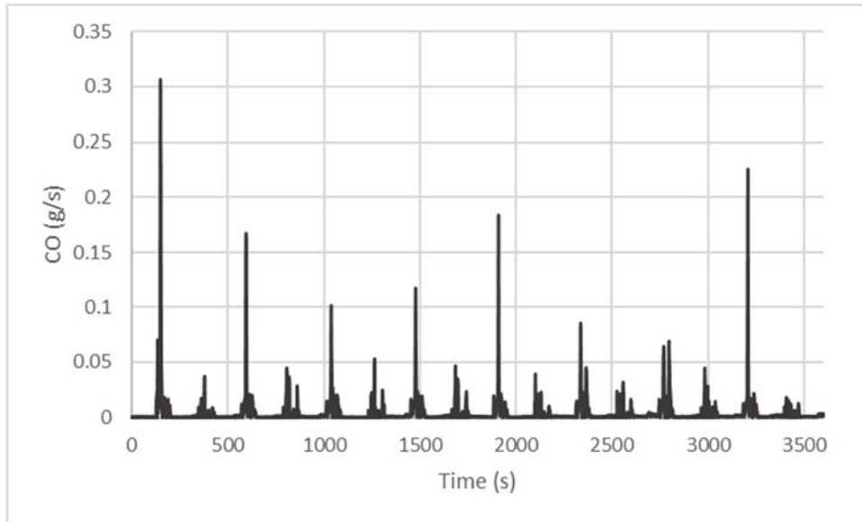
Figure 78: Mass Rate (g/s) of CO Emissions for 2017 Propane School Bus from 2 Minute Stop and Go Route
