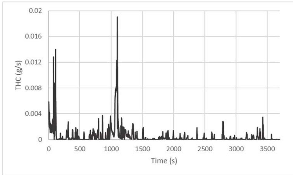
Figure 69: Mass Rate (g/s) of THC Emissions for 2017 Propane School Bus from Hot Morgantown Route
