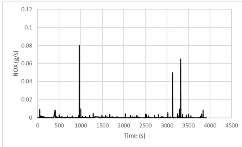
Figure 38: Mass Rate (g/s) of NO x Emissions for Propane School Bus from Cold Morqantown Route
