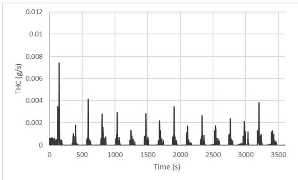
Figure 88: Mass Rate (g/s) of THC Emissions for 2017 Propane School Bus from 2 Minute Stop and Go Route
