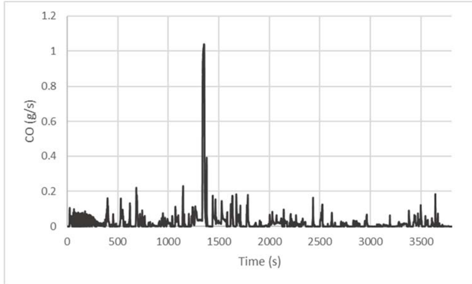
Figure 57: Mass Rate (g/s) of CO Emissions for 2017 Propane School Bus from Cold Morgantown Route
