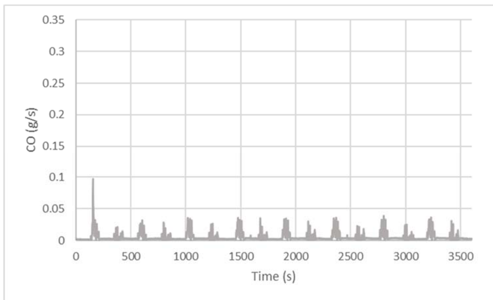
Figure 79: Mass Rate (g/s) of CO Emissions for 2017 Diesel School Bus from 2 Minute Stop and Go Route
