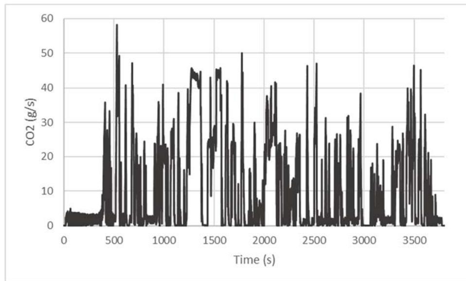
Figure 62: Mass Rate (g/s) of CO 2 Emissions for 2017 Propane School Bus from Cold Morgantown Route
