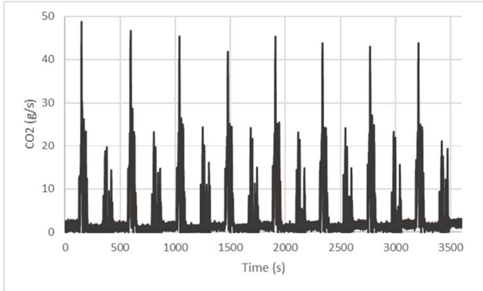
Figure 83: Mass Rate (g/s) of CO 2 Emissions for 2017 Propane School Bus from 2 Minute Stop and Go Route
