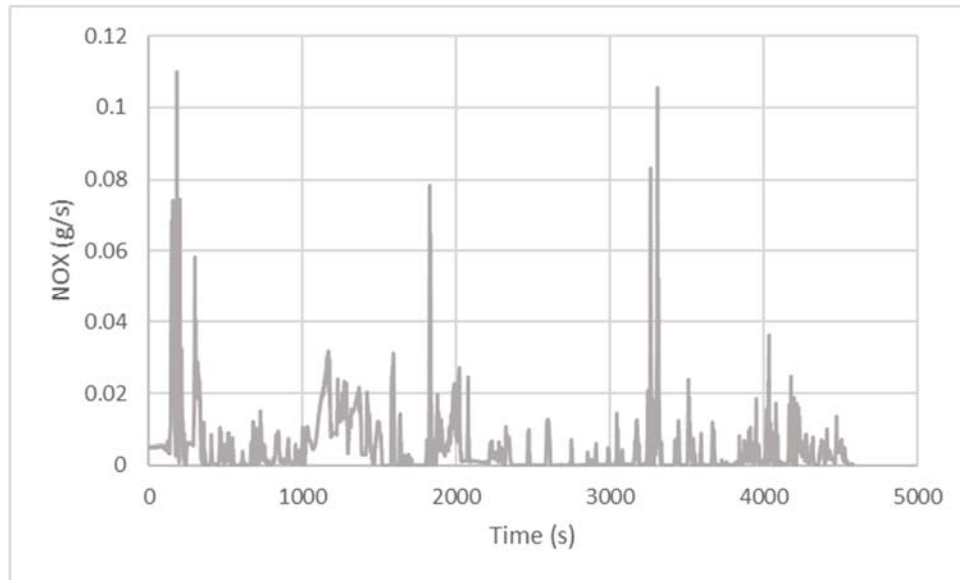
Figure 41: Mass Rate (g/s) of NO x Emissions for Diesel School Bus from Hot Morgantown Route
