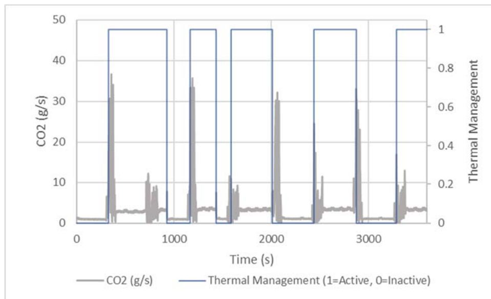
Figure 86: Mass Rate (g/s) of CO 2 Emissions for 2017 Diesel School Bus from 5 Minute Stop and Go Route
