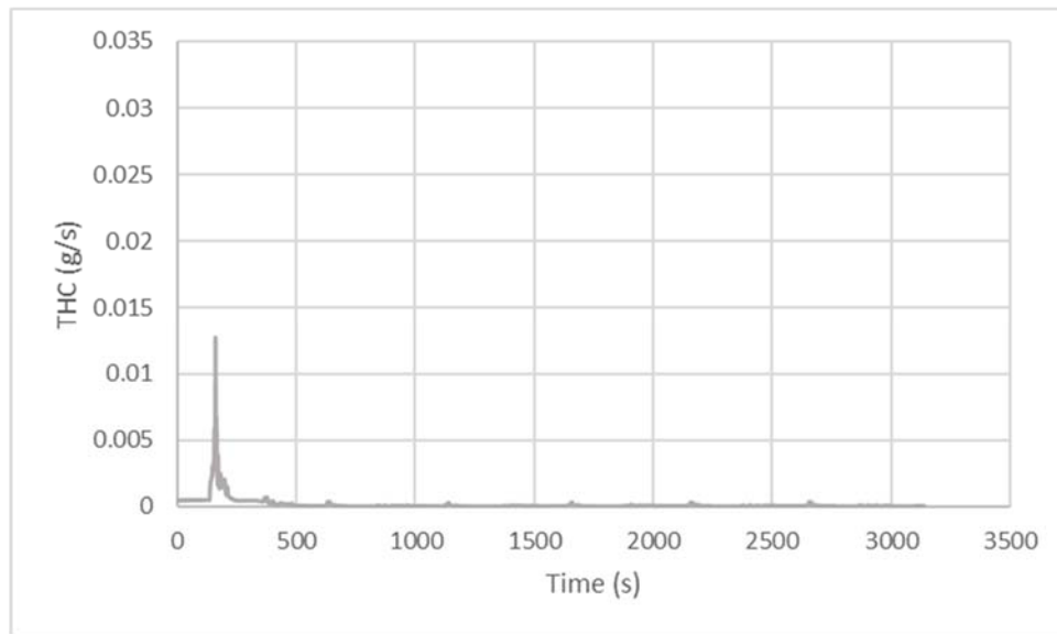
Figure 51: Mass Rate (g/s) of THC Emissions for Diesel School Bus from Stop and Go Route
