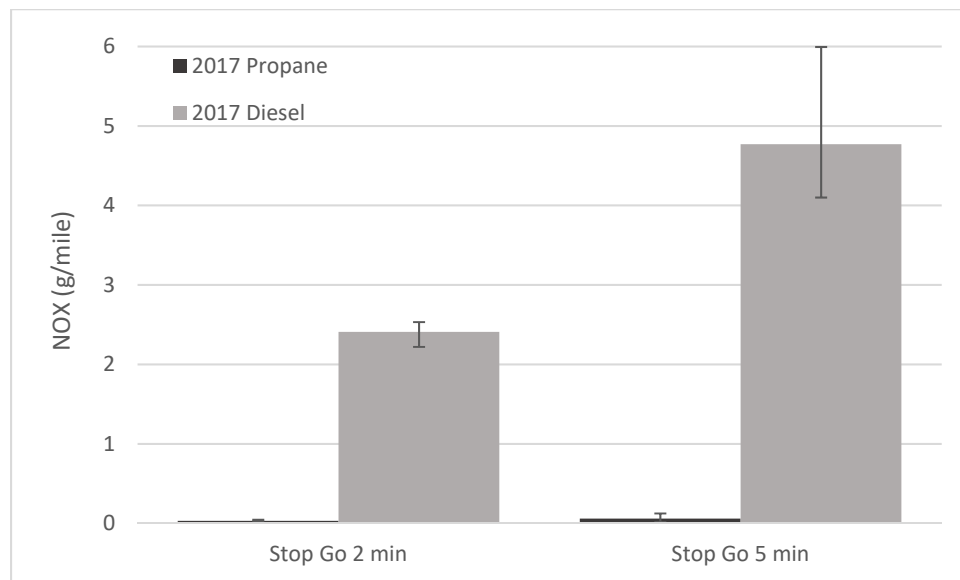
Figure 92: Average NO x Emissions (g/mile) for 2017 Propane and 2017 Diesel School Bus
