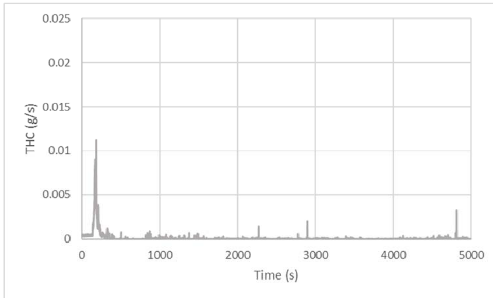
Figure 36: Mass Rate (g/s) of THC Emissions for Diesel School Bus from Hot Morgantown Route
