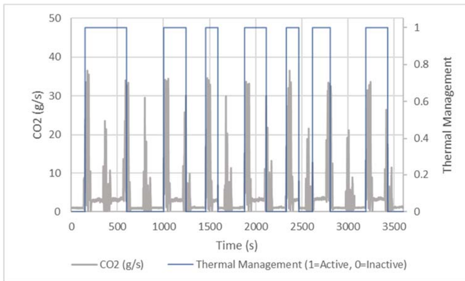
Figure 84: Mass Rate (g/s) of CO 2 Emissions for 2017 Diesel School Bus from 2 Minute Stop and Go Route
