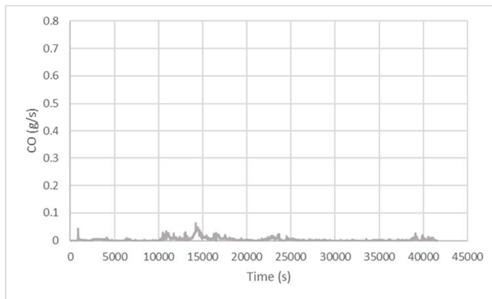
Figure 24: Mass Rate (g/s) of CO Emissions for Diesel School Bus from Cold Morgantown Route
