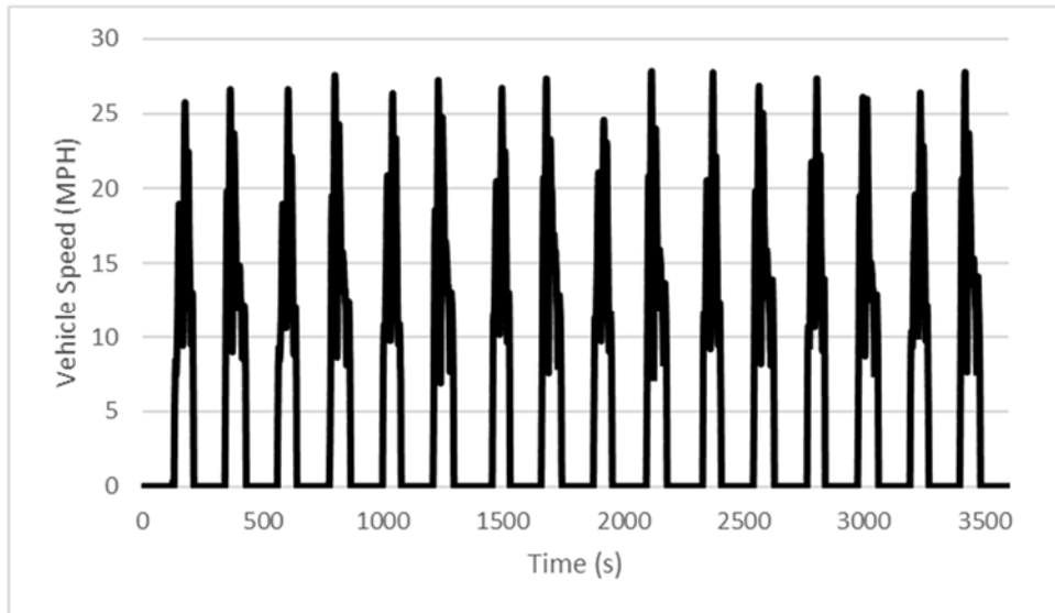
Figure 17: Characteristic Vehicle Speed Trace for the Stop and Go Route (2 Minute)
