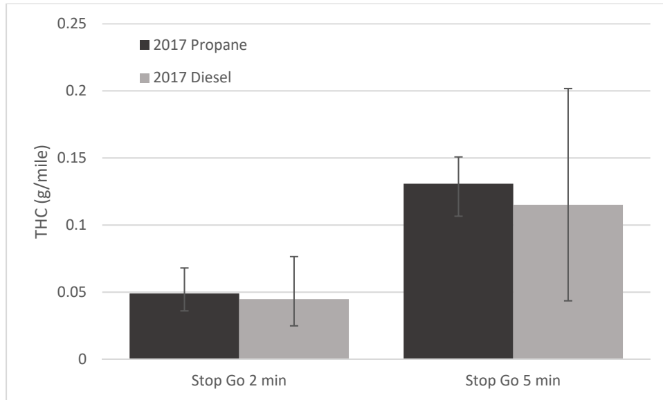
Figure 87: Average THC Emissions (g/mile) for 2017 Propane and 2017 Diesel School Bus
