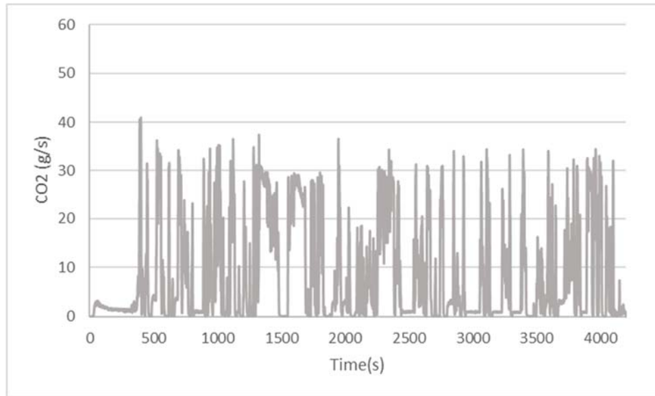
Figure 63: Mass Rate (g/s) of CO 2 Emissions for 2017 Diesel School Bus from Cold Morgantown Route
