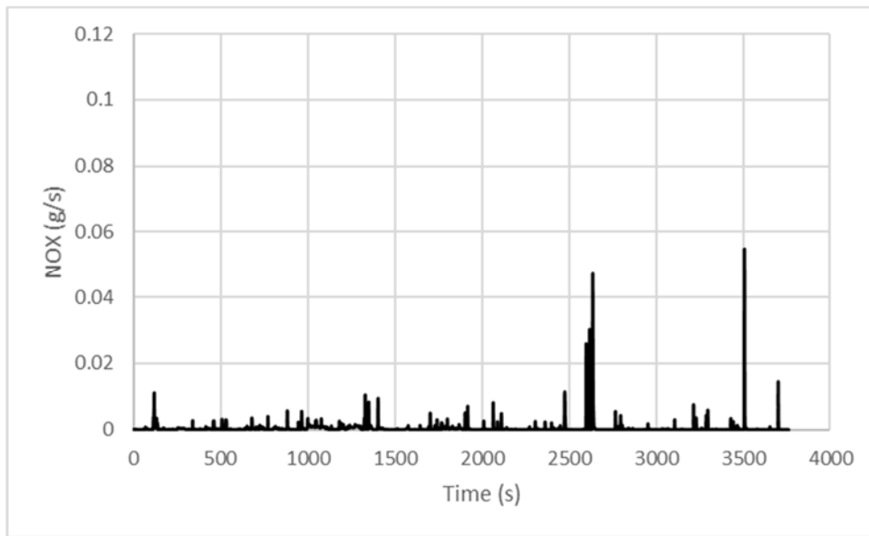
Figure 40: Mass Rate (g/s) of NO x Emissions for Propane School Bus from Hot Morgantown Route
