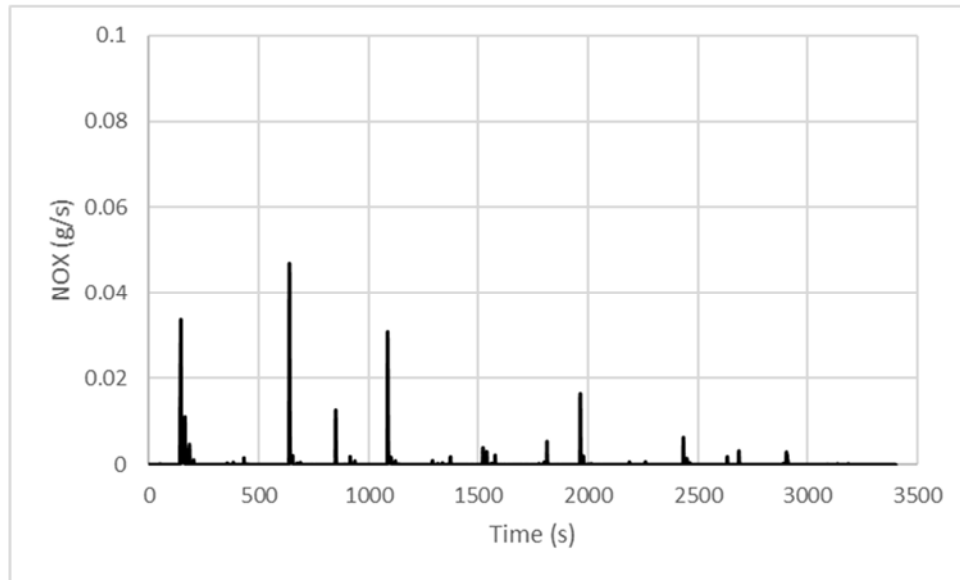
Figure 53: Mass Rate (g/s) of NO x Emissions for Propane School Bus from Stop and Go Route
