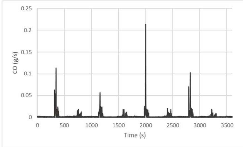
Figure 80: Mass Rate (g/s) of CO Emissions for 2017 Propane School Bus from 5 Minute Stop and Go Route
