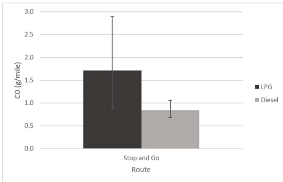
Figure 43: Average CO Emissions (g/mile) for Propane and Diesel School Bus
