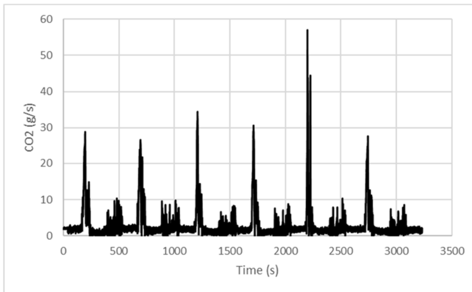
Figure 47: Mass Rate (g/s) of CO 2 Emissions for Propane School Bus from Stop and Go Route
