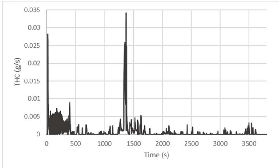
Figure 67: Mass Rate (g/s) of THC Emissions for 2017 Propane School Bus from Cold Morgantown Route
