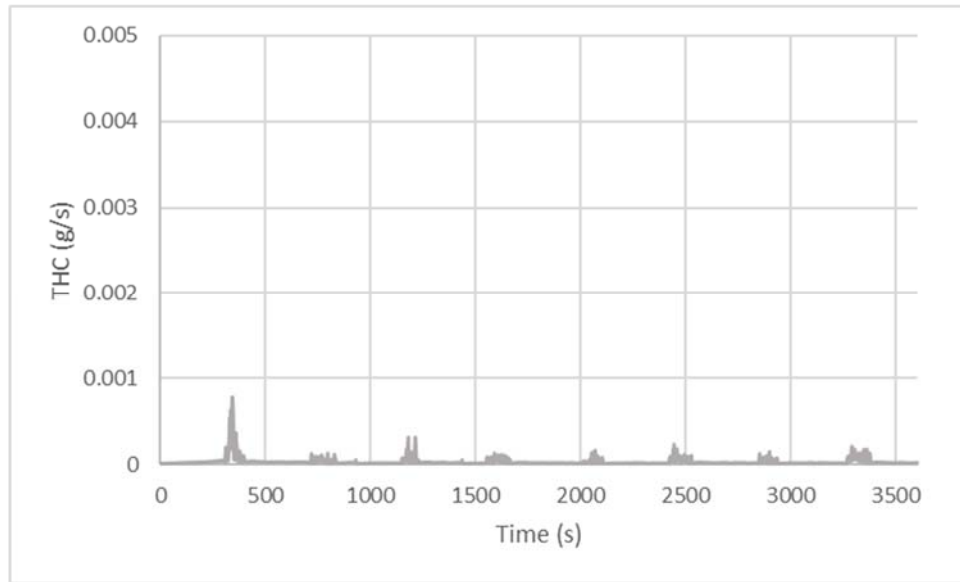
Figure 91: Mass Rate (g/s) of THC Emissions for 2017 Diesel School Bus from 5 Minute Stop and Go Route
