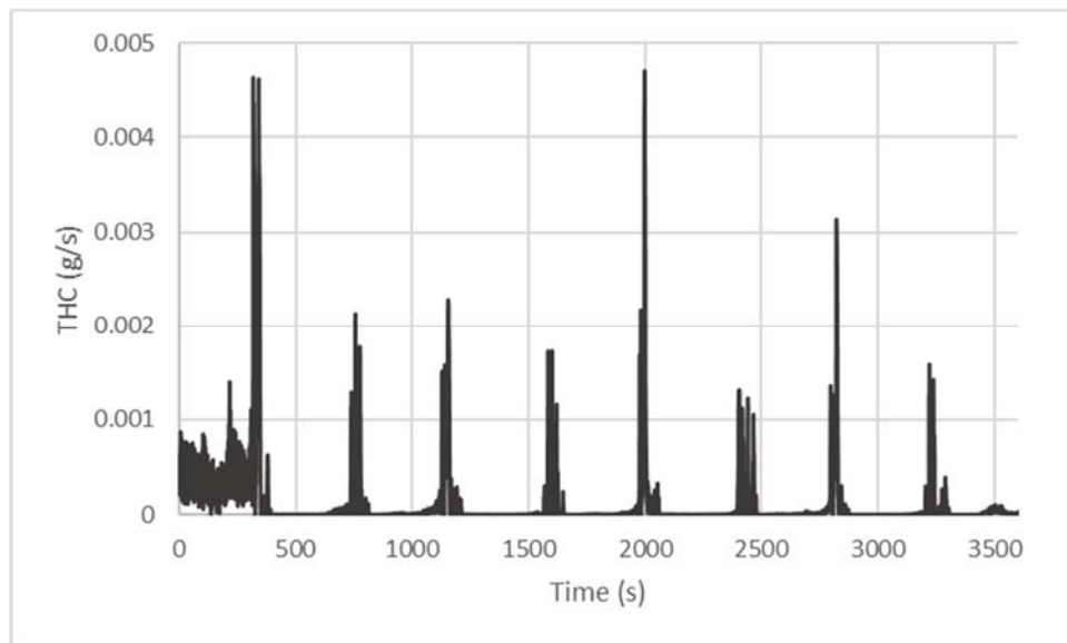
Figure 90: Mass Rate (g/s) of THC Emissions for 2017 Propane School Bus from 5 Minute Stop and Go Route
