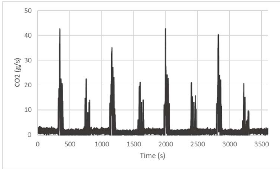
Figure 85: Mass Rate (g/s) of CO 2 Emissions for 2017 Propane School Bus from 5 Minute Stop and Go Route
