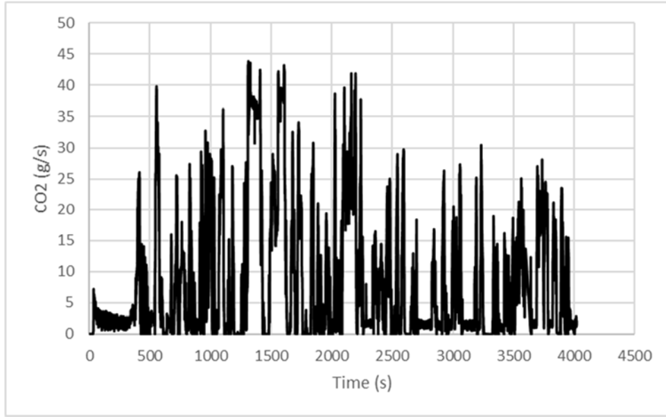
Figure 28: Mass Rate (g/s) of CO 2 Emissions for Propane School Bus from Cold Morgantown Route
