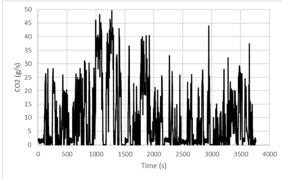
Figure 30: Mass Rate (g/s) of CO 2 Emissions for Propane School Bus from Hot Morgantown Route
