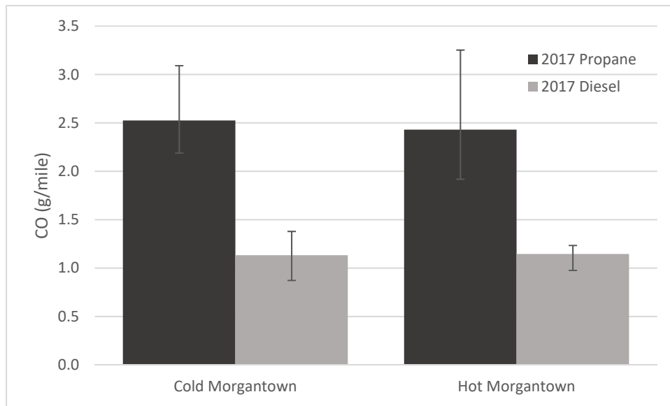
Figure 56: Average CO Emissions (g/mile) for 2017 Propane and 2017 Diesel School Bus
