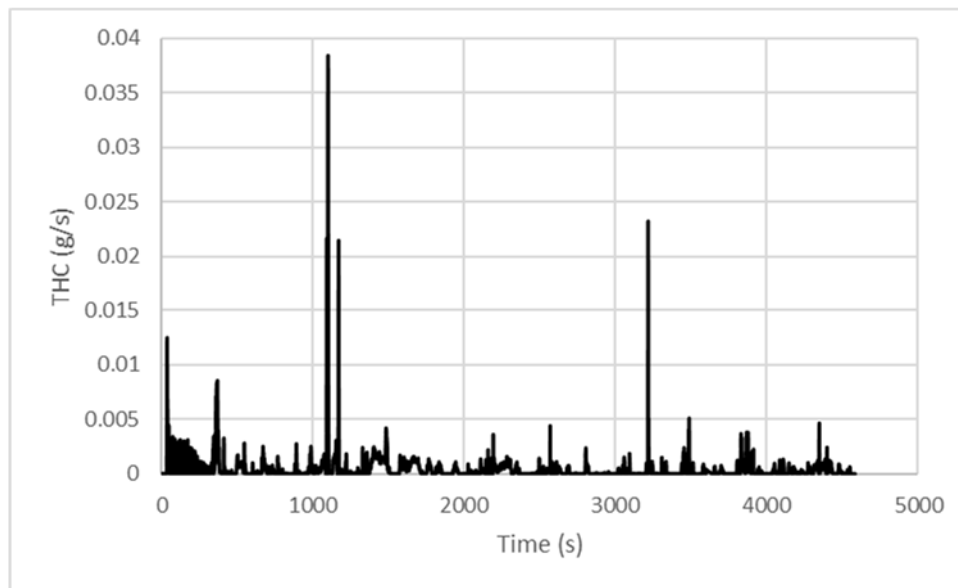
Figure 33: Mass Rate (g/s) of THC Emissions for Propane School Bus from Cold Morqantown Route
